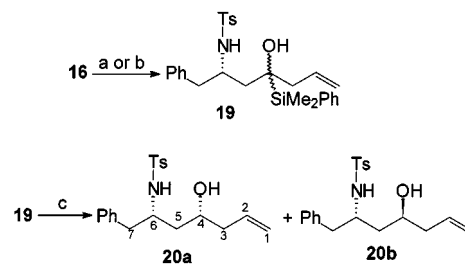
Scheme 8. a) allyltrimethylsilane, TiCl 4 (1 equiv.), –78°C, 24 h, de 64%, 62%; b) tetraallyltin (0.5 equiv), Sc(OTf) 3 (7 mol-%), 20°C, 24 h, de 50%, 96%; c) TBAF, THF, r.t., 72 h, starting from 19 de 50%, 72%
