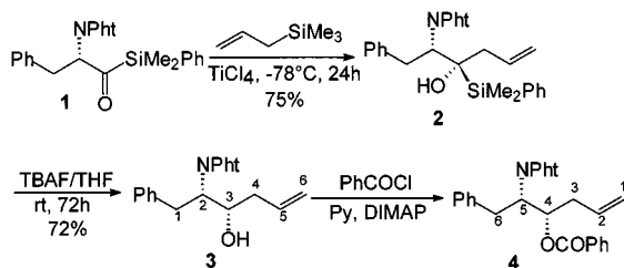
Scheme 1. Synthesis of (2 S ,3 S )-1-phenyl-2-phthalimido-5-hexen-3-ol 3 and its conversion into the benzoyl derivative 4
