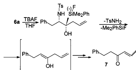
Scheme 3. Reaction of 6a with TBAF
