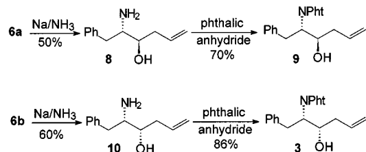
Scheme 4. Deprotection and desilylation of 6a and 6b , followed by transformation of 8 and 10 into the phthaloyl derivatives 9 and 3
