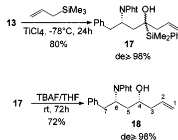
Scheme 7. Synthesis of (4 R ,5 R )-7-phenyl-6-phthalimido-1-hepten-4-ol 18
