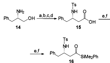
Scheme 6. a) TsCl, THF/H 2 O, r.t., 9 h, 98%; b) Ph 3 P, I 2 , imidazole, CH 3 CN, 95–100°C, 1 h, 90%; c) Bu 4 CN, CH 3 CN, 70°C, 4 h, 65%; d) H 2 SO 4 , CH 3 COOH, H 2 O, 110°C, 9 h, 70%; e) SOCl 2 , 55–60°C, 6 h, 95%; f) (PhMe 2 Si) 2 CuCN(Li) 2 , –78°C, 1 h, 50%
